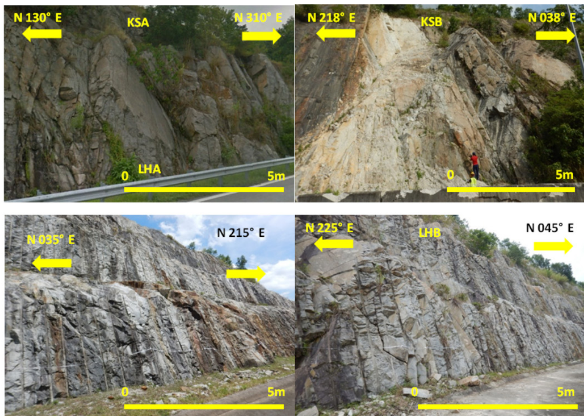
FIGURE 5. Field photo for Slope KSA, KSB, LHA, and LHB. All slopes studied were granite rock cut slopes
