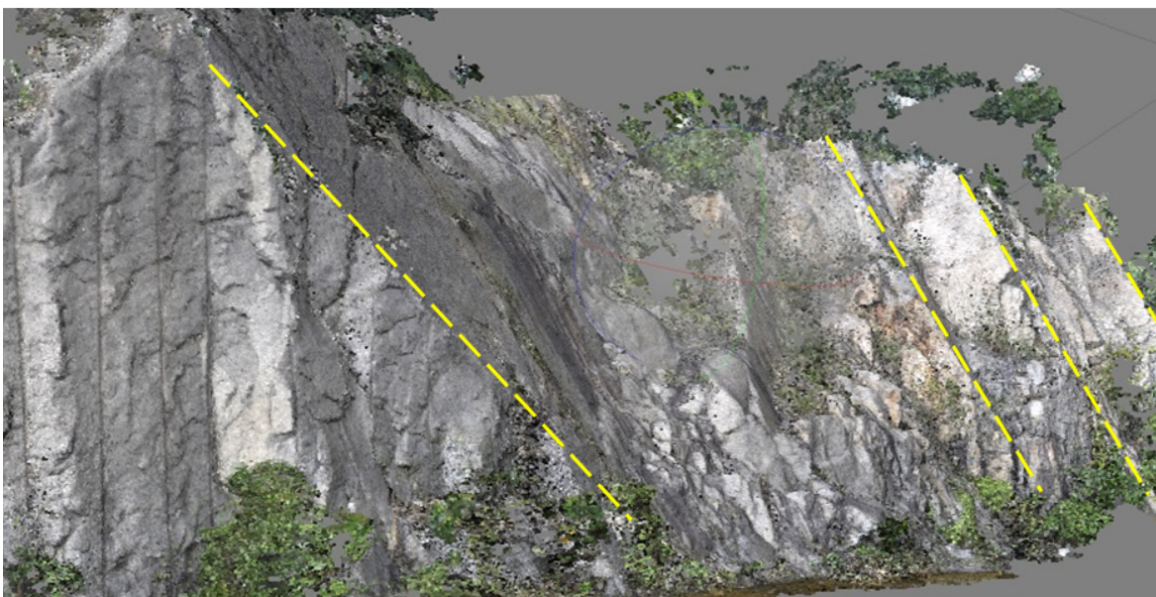
FIGURE 4. The point cloud model obtained from photogrammetry survey of Slope KSA, showing signs of relic planar failure as shown in yellow dashed lines
